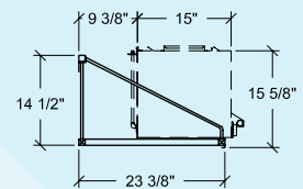
EXTENDED WALL MOUNT
