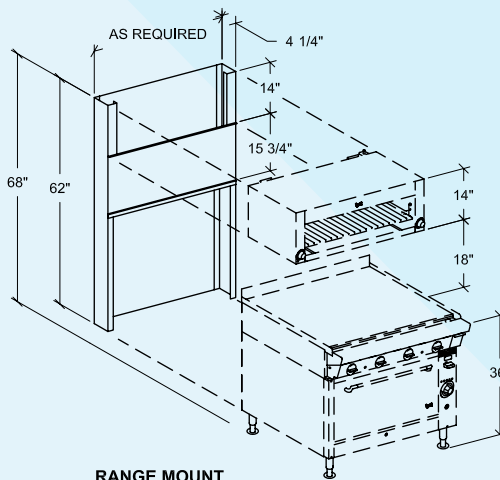
RANGE MOUNT
