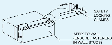
WALL MOUNT REAR VIEW
