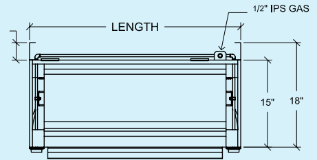
PLAN VIEW
