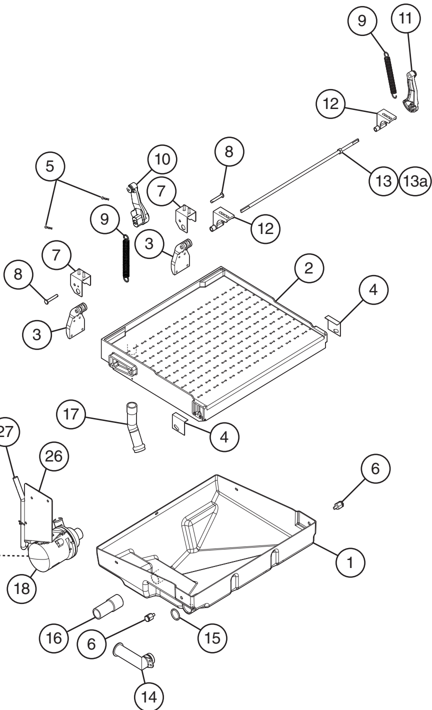
Mechanism Assembly
