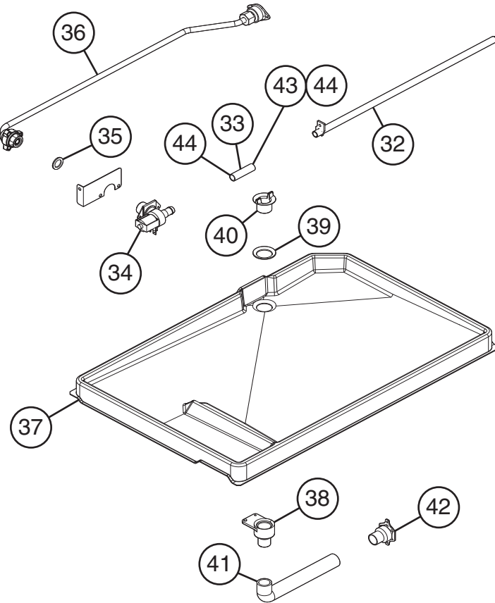
Water Circuit
