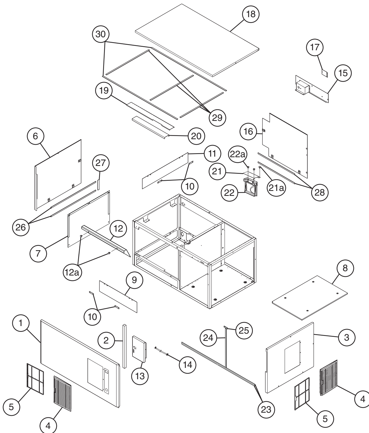
Main Assembly
