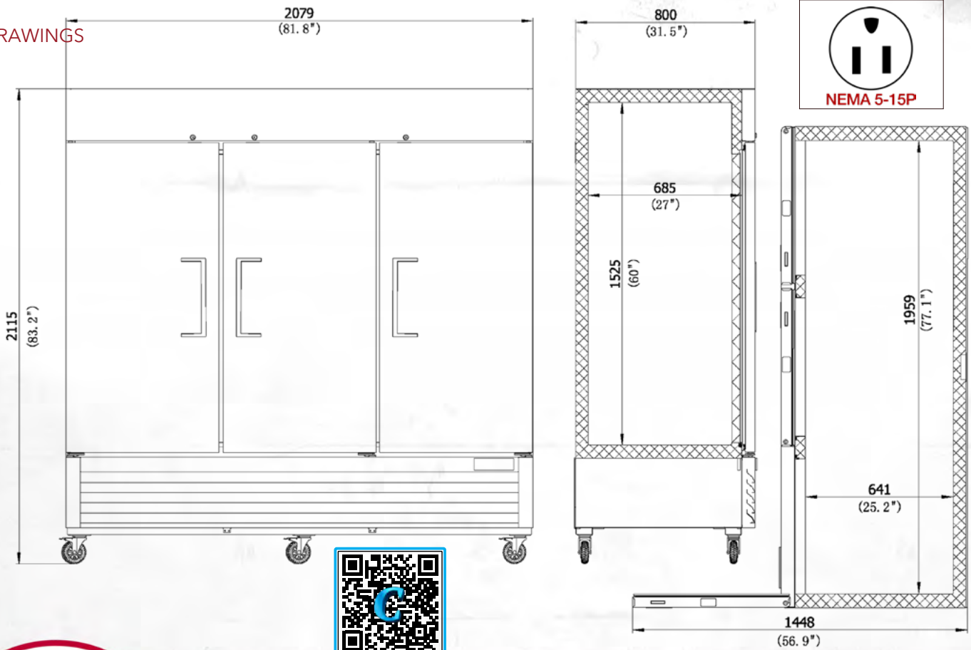
PRODUCT DRAWINGS
