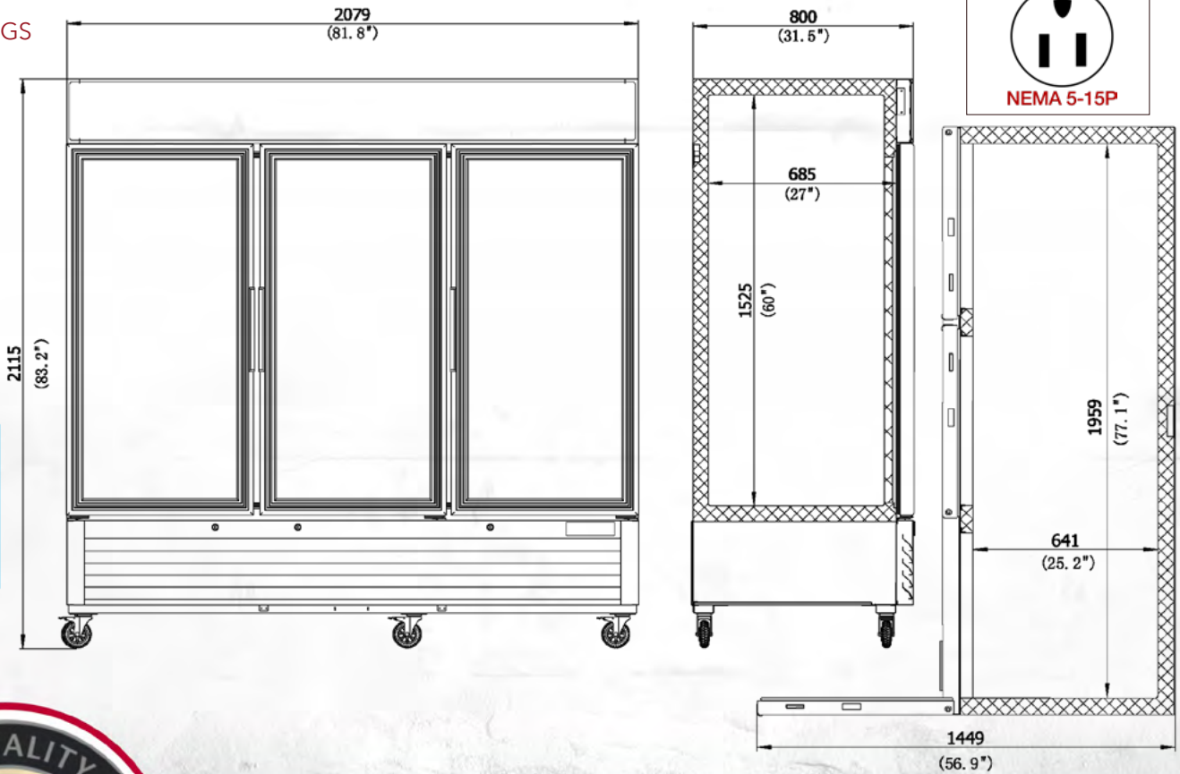
PRODUCT DRAWINGS
