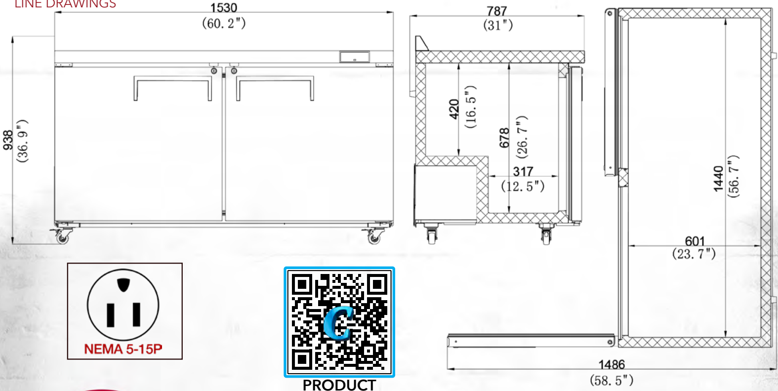
PRODUCT DRAWINGS
