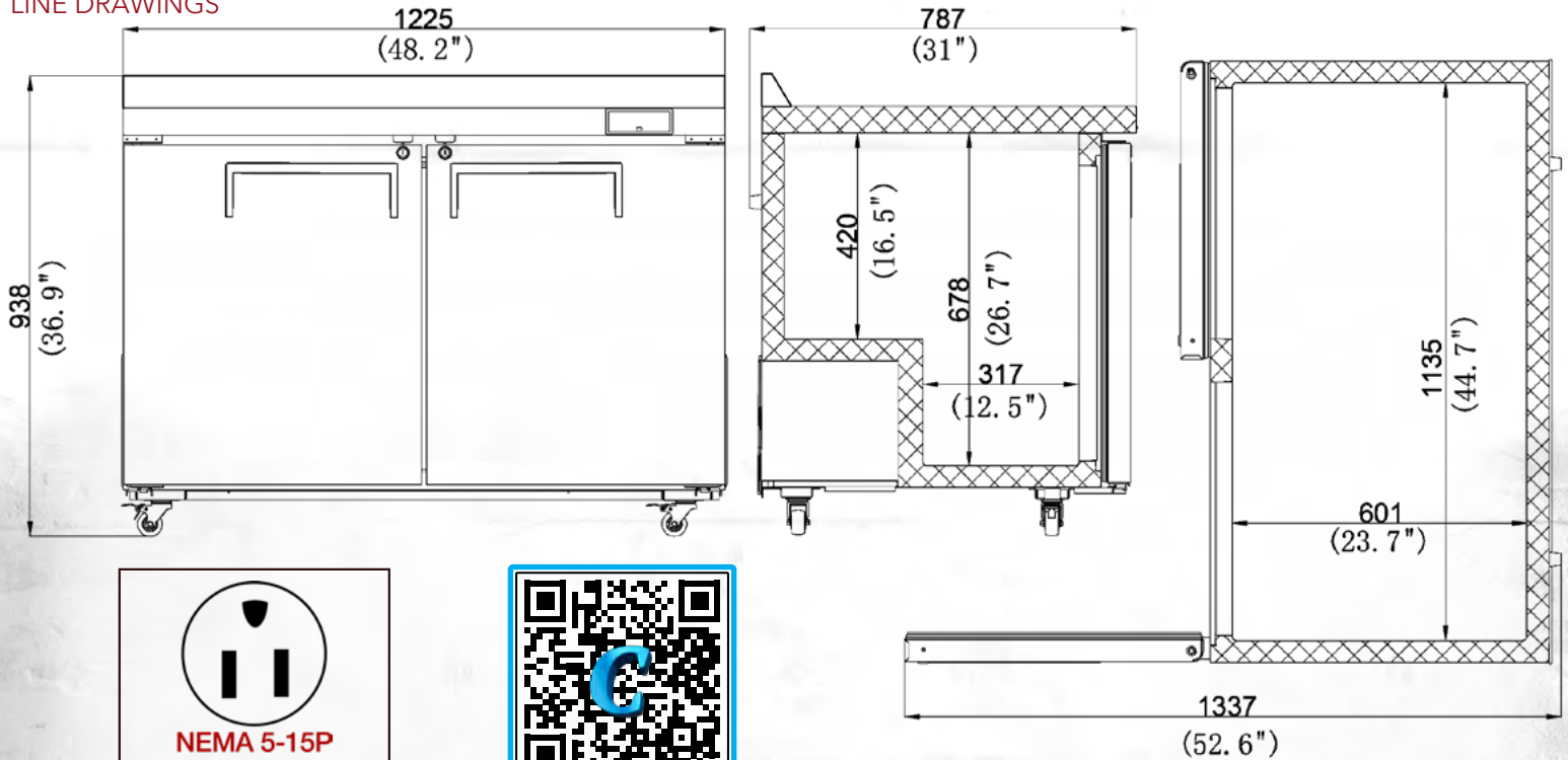
PRODUCT DRAWINGS
