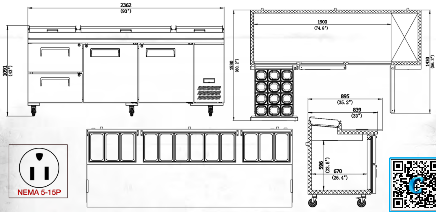
PRODUCT DRAWINGS
