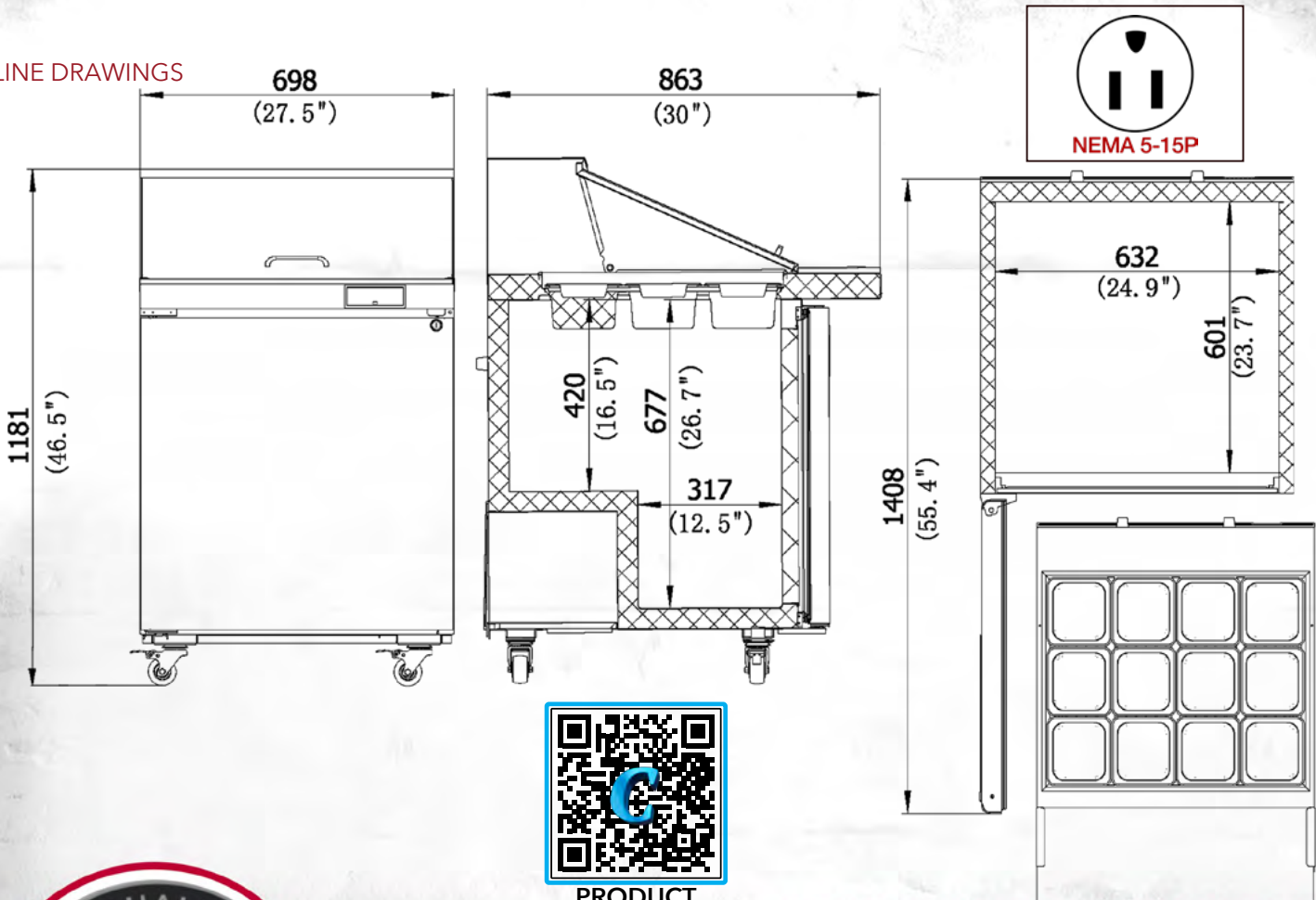
PRODUCT DRAWINGS
